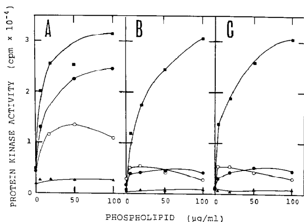
Fig.1. The activation of three types of PKC by various concentrations of phospholipids. PKC was assayed with 3 \mu\text{M} \text{CaCl}_2 , 0.8 \mu\text{g/ml} 1,2-diolein, and various concentrations of each phospholipid as described in section 2. (A) Type I; (B) type II; (C) type III. (●) Phosphatidylethanol; (○) phosphatidylmethanol; (■) phosphatidylserine; (▲) phosphatidylethanolamine.
